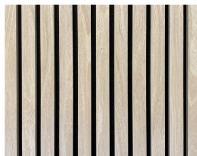
Z-UP SPILEPANEL GLOMMA 2700x600x24mm 1,62m 2 15 spiler Art.nr: 600070
