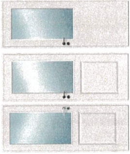
Light internal doors with glass $ moulded, non-rebated, rebated or flush
